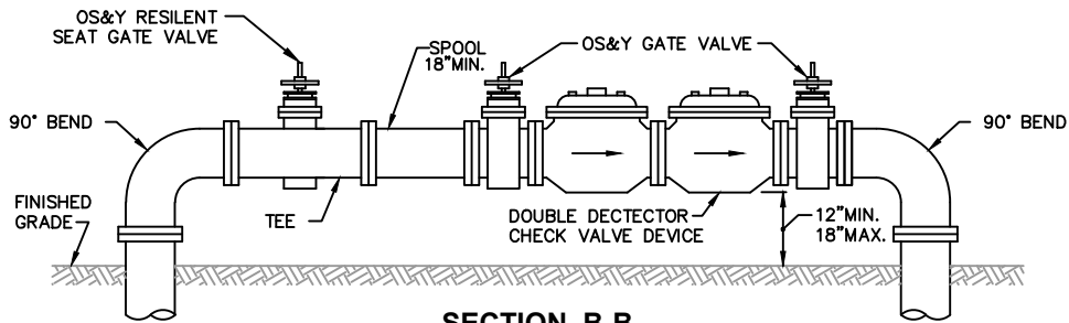
SECTION B-B (FIRE SERVICE PORTION)
