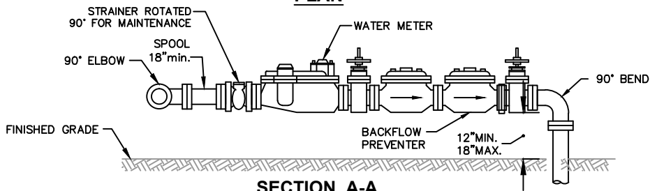
SECTION A-A (DOMESTIC SUPPLY PORTION)
